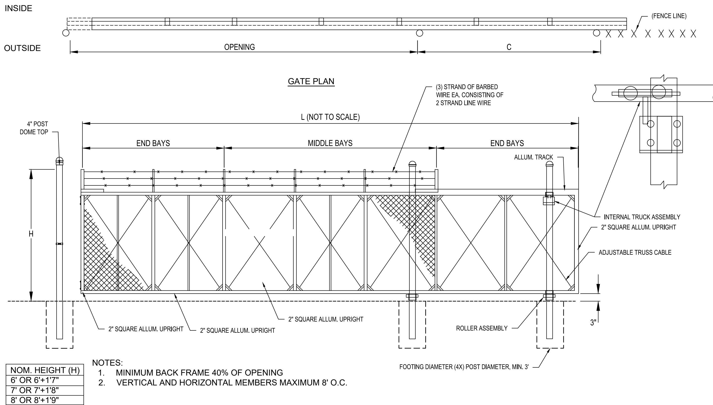
SINGLE CANTILEVER SLIDING GATE ROUND POSTS W/ BARBED WIRE (10' - 30' OPENINGS) NOT TO SCALE
